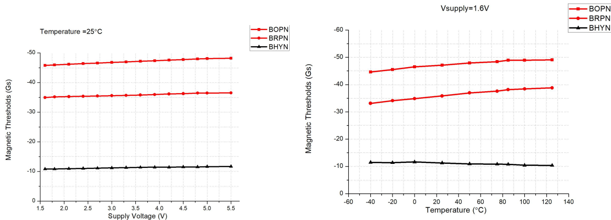
Magnetic Thresholds vs. Supply Voltage @ T_A = 25^\circ C
