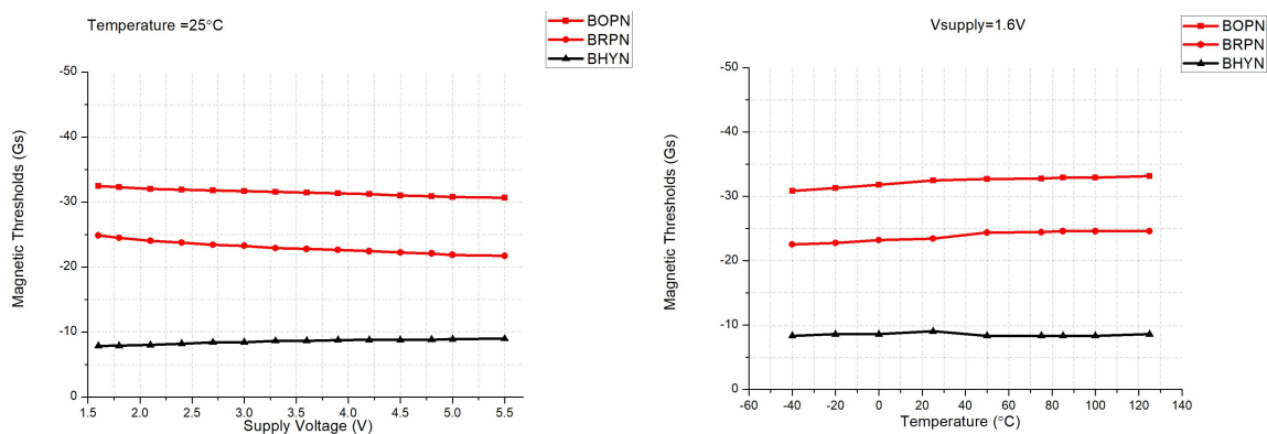
Magnetic Thresholds vs. Supply Voltage @ T_A = 25^\circ C
