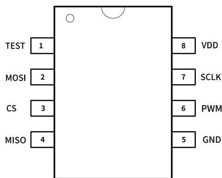
图 4: SOP-8 4.9mmx6mm
